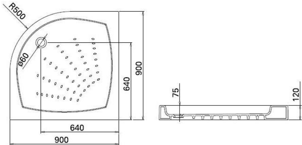
107051 Aresta Shower Tray 900 X 900 X 120
